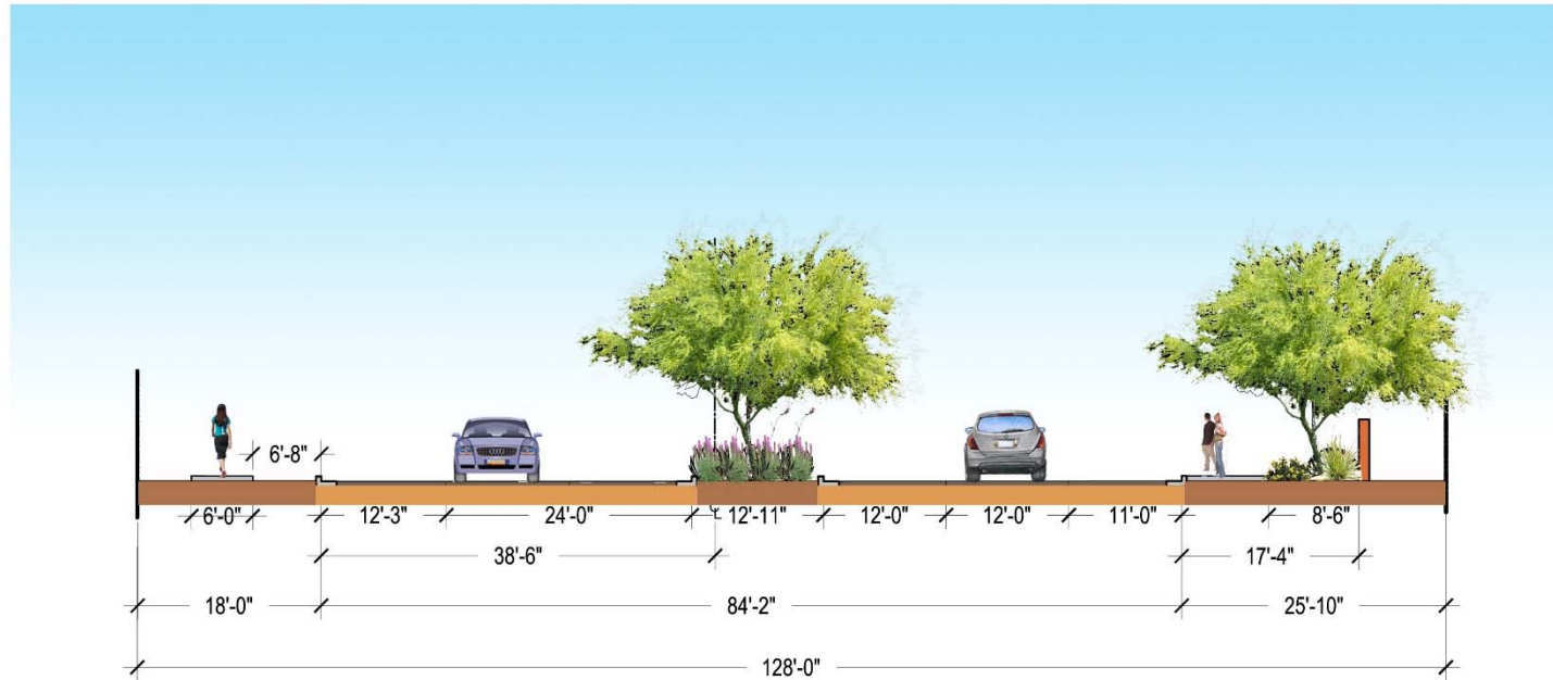
PROPOSED McDOWELL ROAD SECTION AT STATION 90+00
