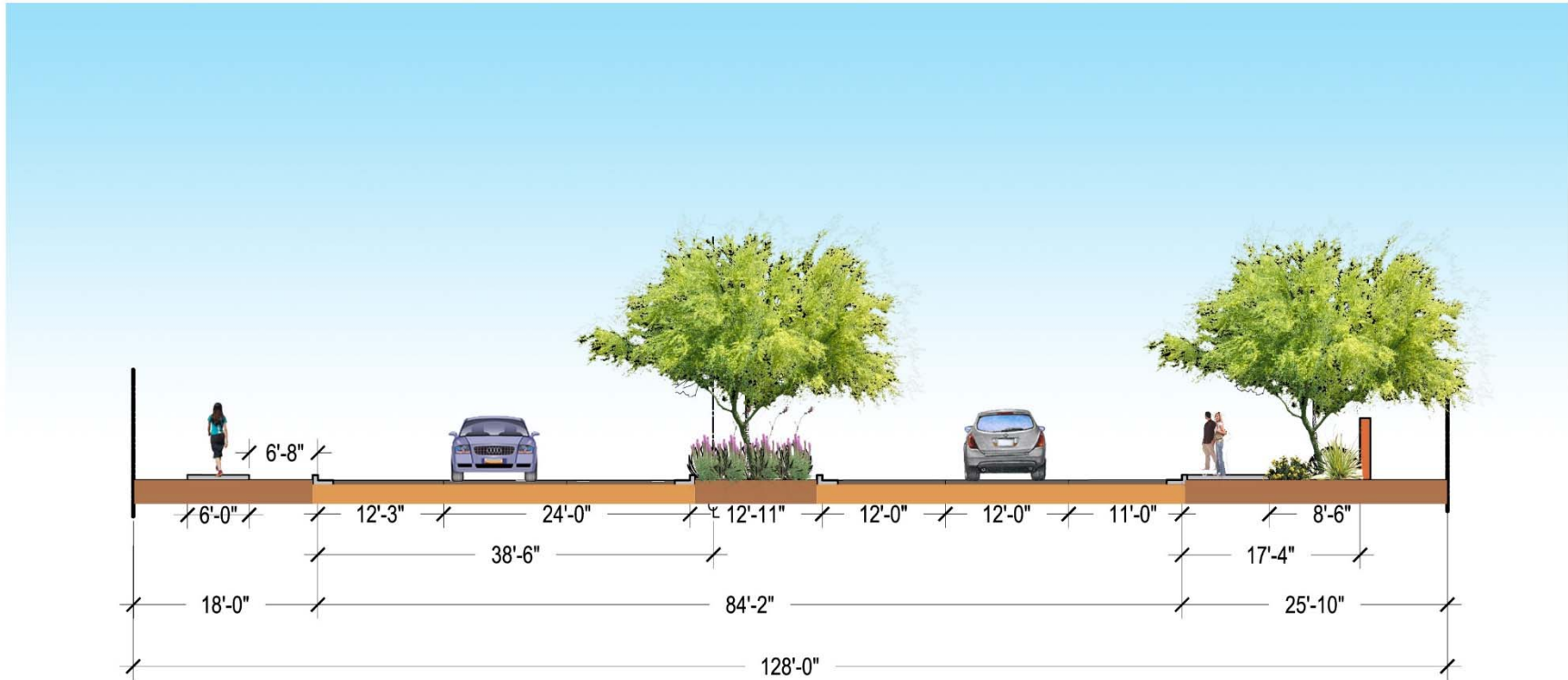
PROPOSED McDOWELL ROAD SECTION AT STATION 90+00
