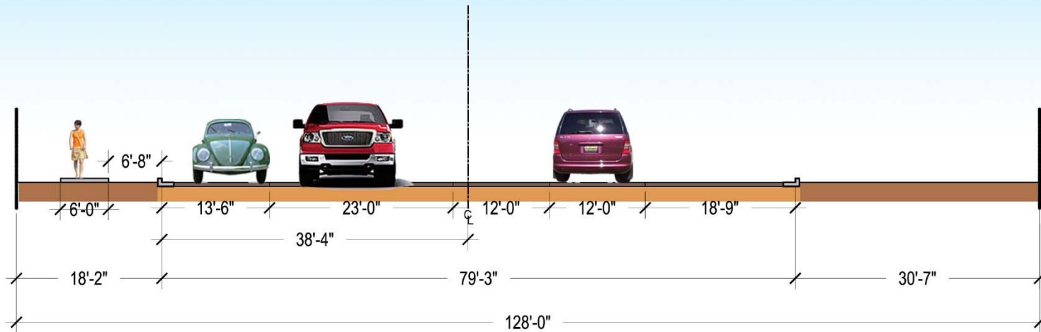
EXISTING McDOWELL ROAD SECTION AT STATION 90+00
