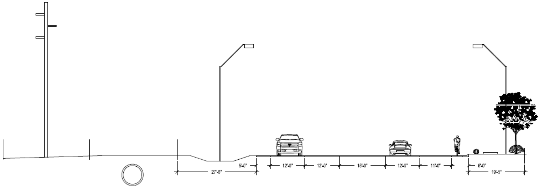
107TH AVENUE TYPICAL SECTION
